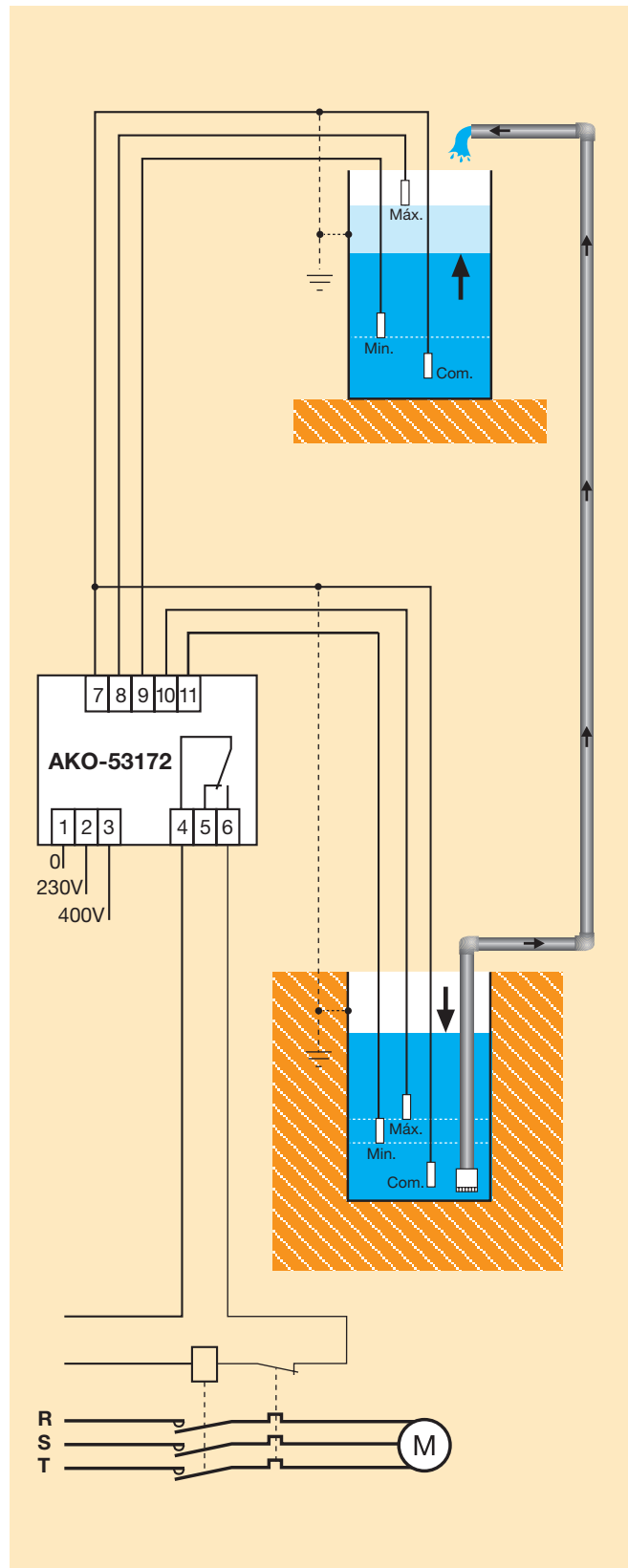
Trasvase entre pozo y depósito Transfer between well and tank
