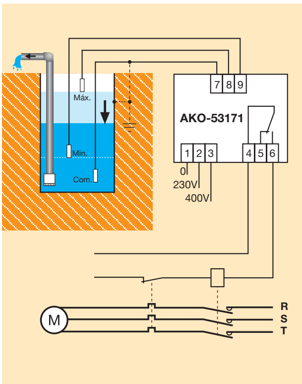
Vaciado (pozo) Draining (well)
